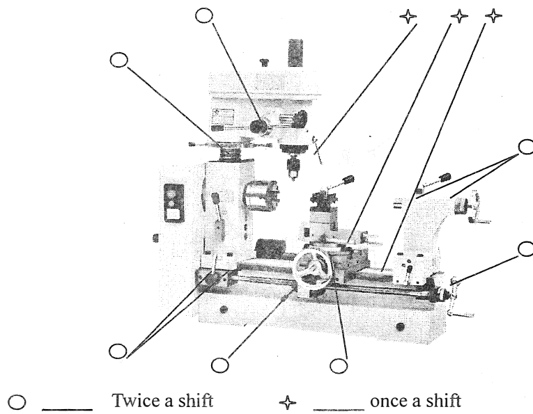
Fig.4.Lubrication chart
