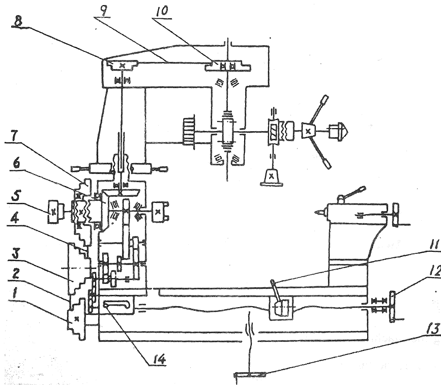
Fig.5 Transmission system
